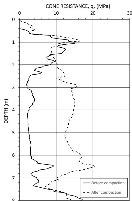
Figure 9a Cone resistance prior to, and after resonance compaction, Antwerp
