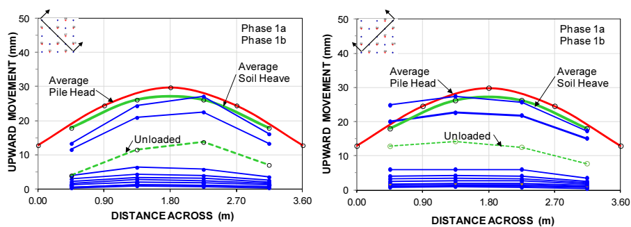
Figure 12. Upward movement of the ground surface within the pile group. Phase 1b.
