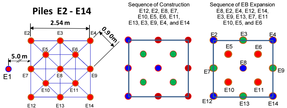
Figure 6. Pile locations and sequence of construction and EB expansion.
